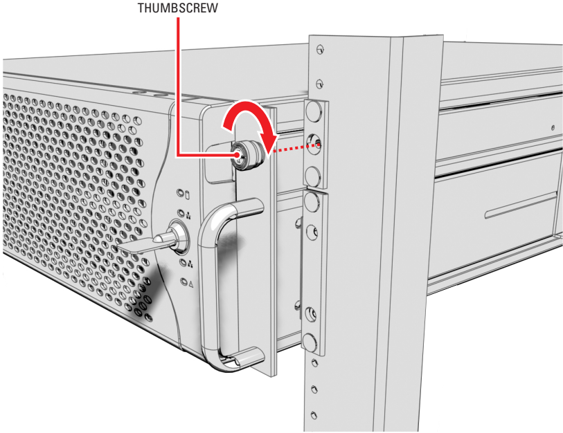
Figure 15. Tightening the Thumbscrews
